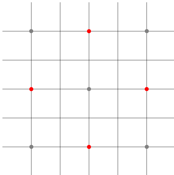
Figure 348: How the diamond-square algorithm works (3/5)
